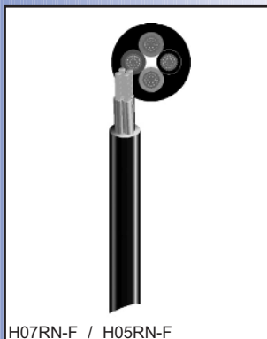
H07RN-F / H05RN-F
